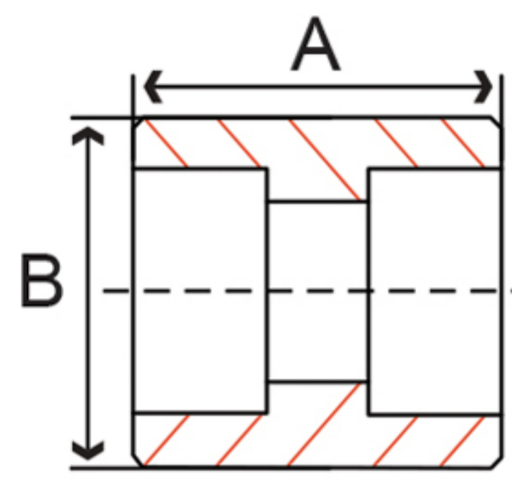
Fig. 52CP3 – Coupling
